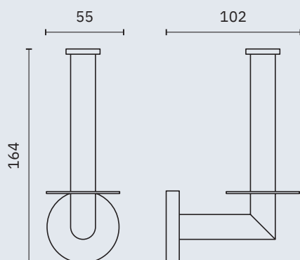
Spare toilet paper roll holder
