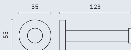
Toilet paper roll holder
